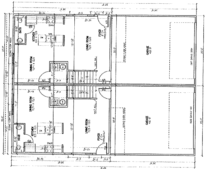
FLOOR PLAN 1/4"=1'-0" 560 SF
