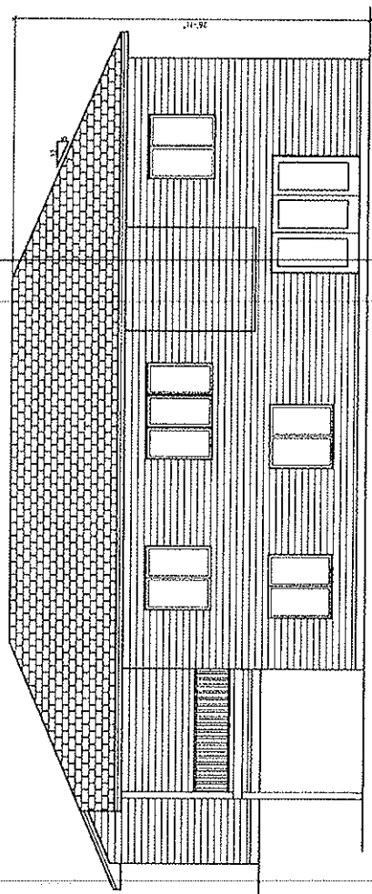
REAR ELEVATION 1/8"=1'-0"
