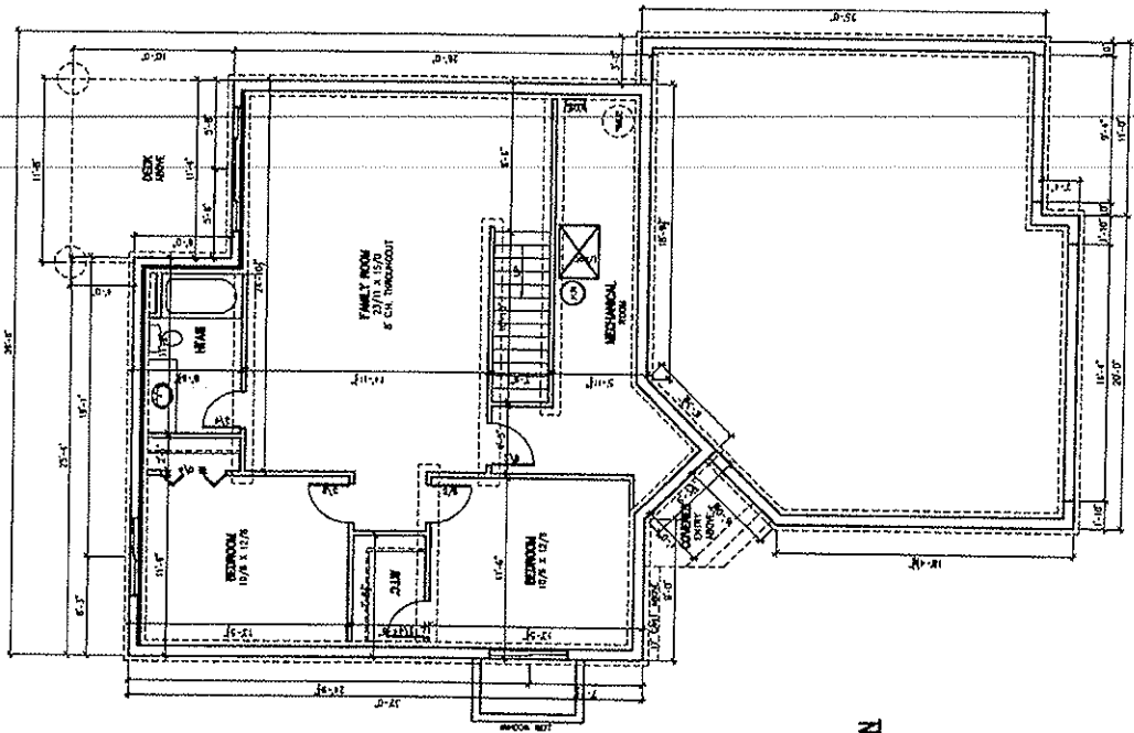
FOUNDATION PLAN 1/8"=1'-0" 846 SF
