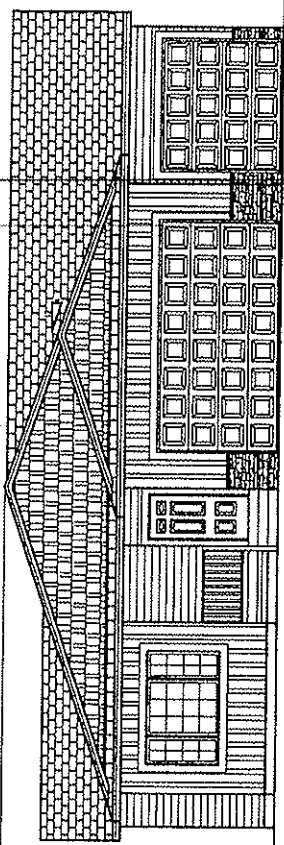
FRONT ELEVATION 1/8"=1'-0"
