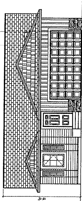
FRONT ELEVATION 1/8"=1'-0"
